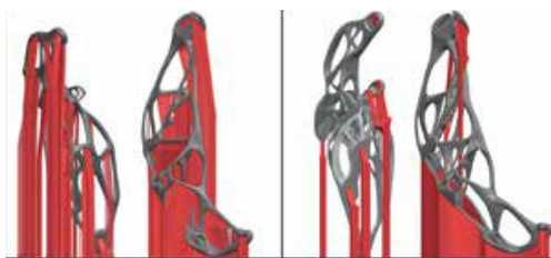
Fig. 2 Minimization of the support structures with more than 50% (left) and less than 30% of the material volume © EDAG
