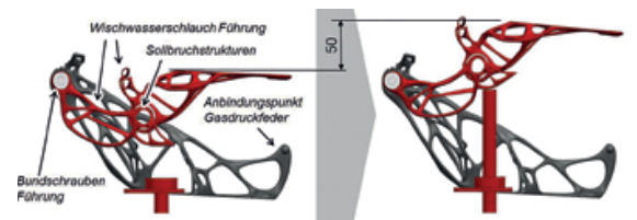
Fig. 3 Functional integration of components; operating principle of additively manufactured predetermined breaking point structures (detail, right) © EDAG
